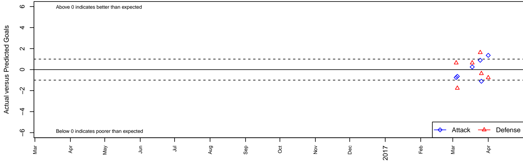
MIFC White G05 Dots are actual minus expected GF (blue circles) and GA (red triangles). Blue line is smoothed change in attack strength. Red is smoothed change in defense strength.
